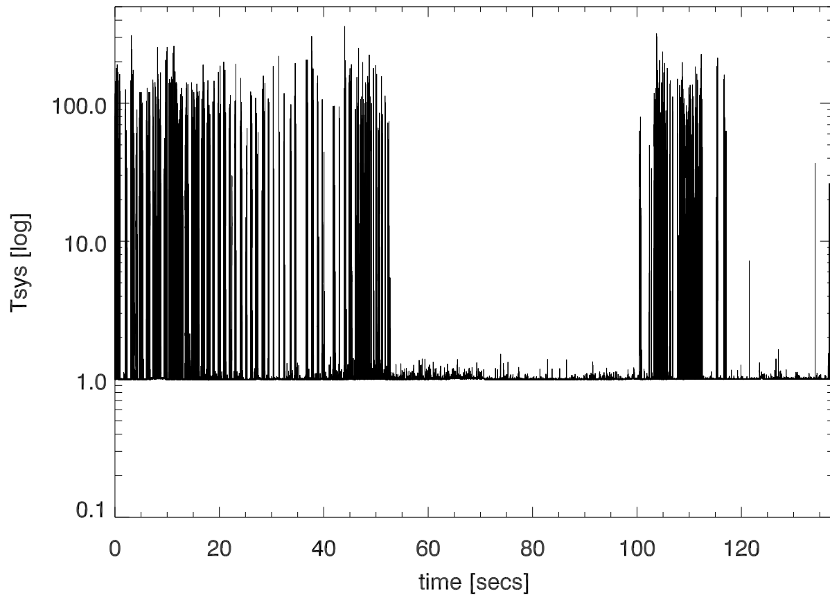
06may15. 327 rcvr total pwr vs time showing glitches.
