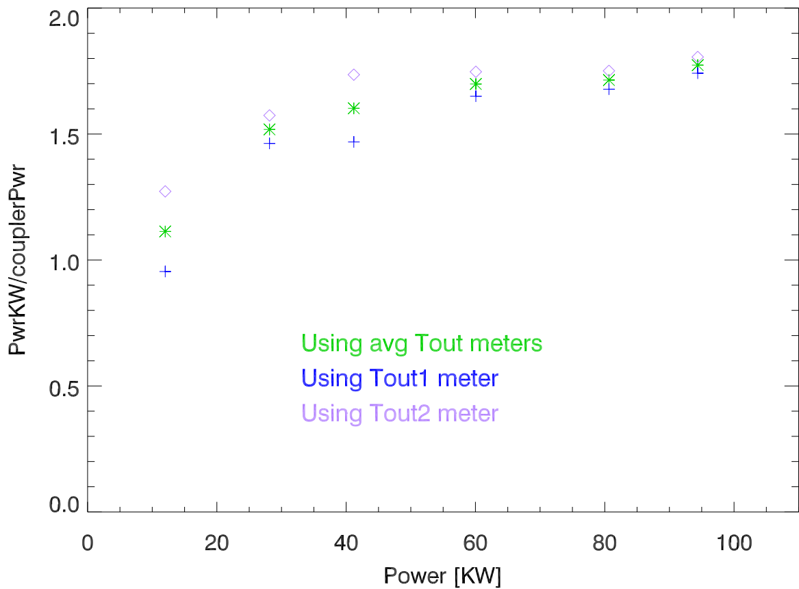
Ratio PwrKw/couplerPwrLin
