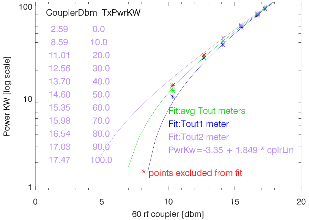
tx6 output power vs rf Coupler
