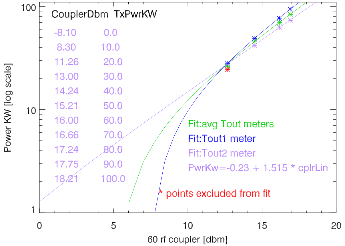
tx1 output power vs rf Coupler
