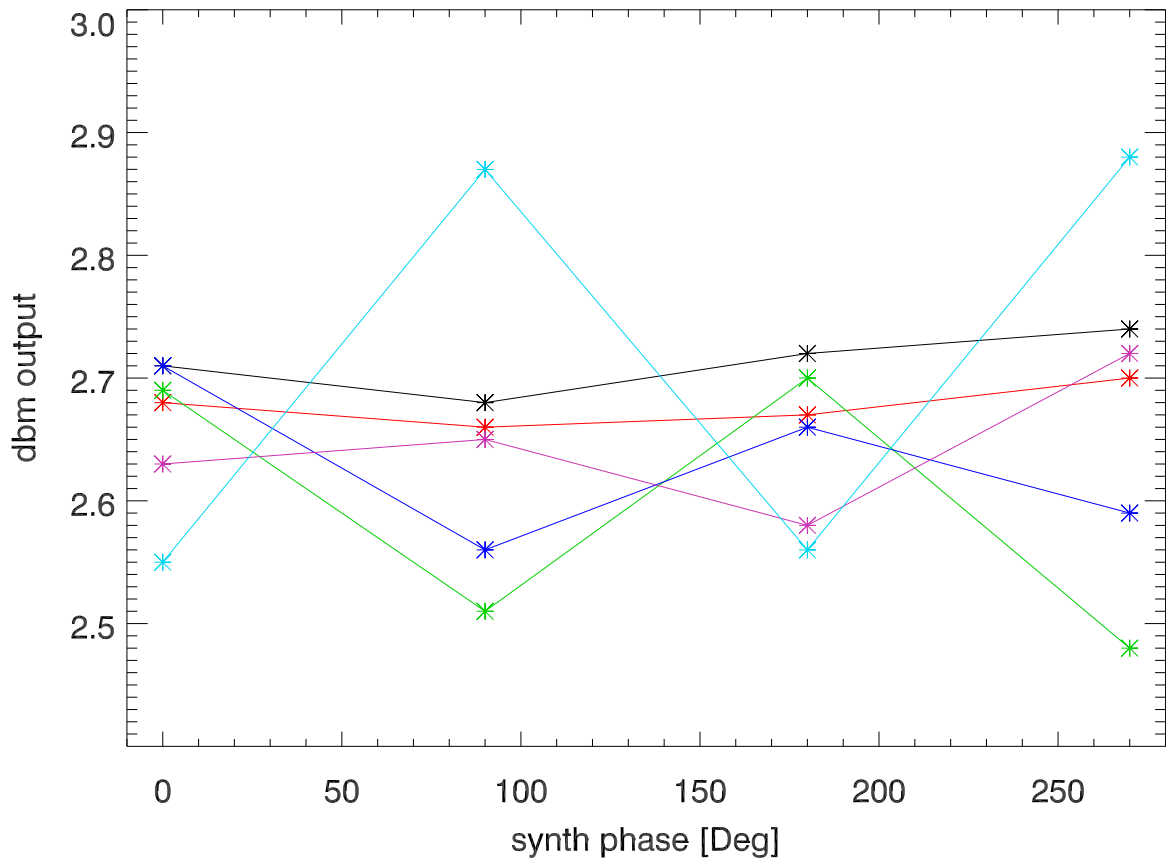
dbm Output vs synth Phase for 0dbf output
