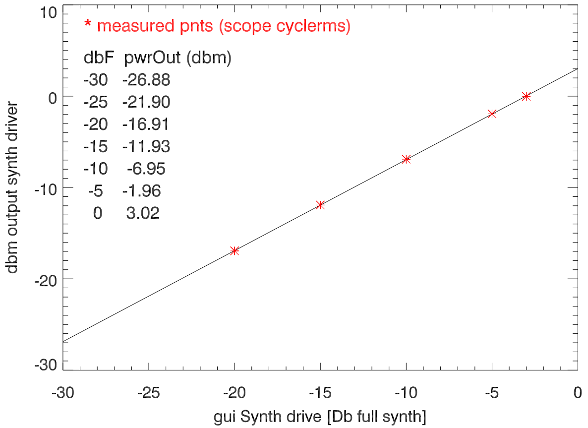
151020 synth driver output pwr vs gui dbFullScale
