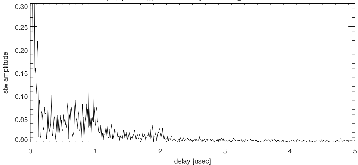
abs(fft(spcMax)) stw vs delay for strongest burst.PoIA
