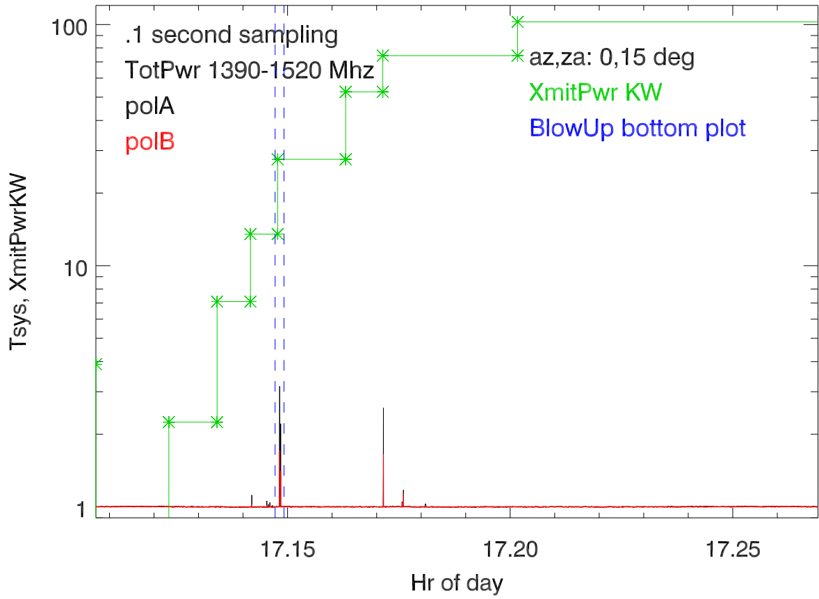
02jun15 Alfa bm0 totPwr vs time. hf Tx6 on antenna
