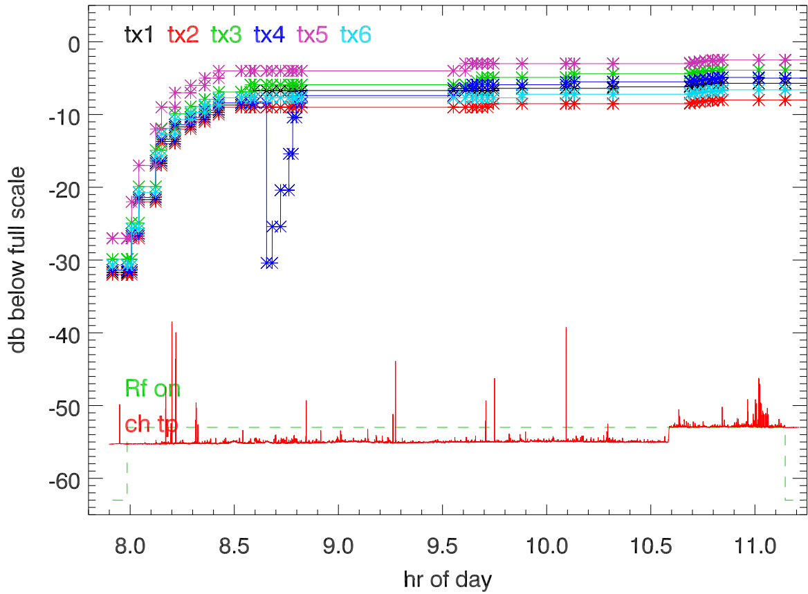
160527 on Antenna. synth drive amplitude
