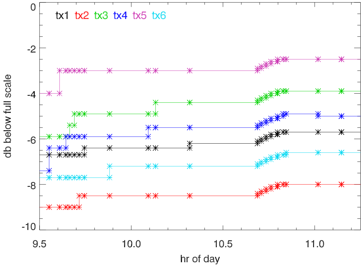
160527 on Antenna. Blowup. synth drive amplitude
