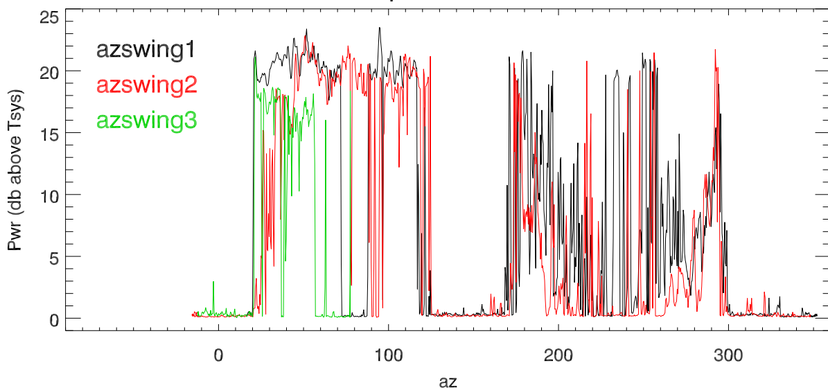
02nov11 HfOn. totpwr vs azimuth. Dome za=15.
