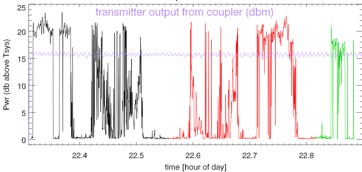
totpwr vs time.
