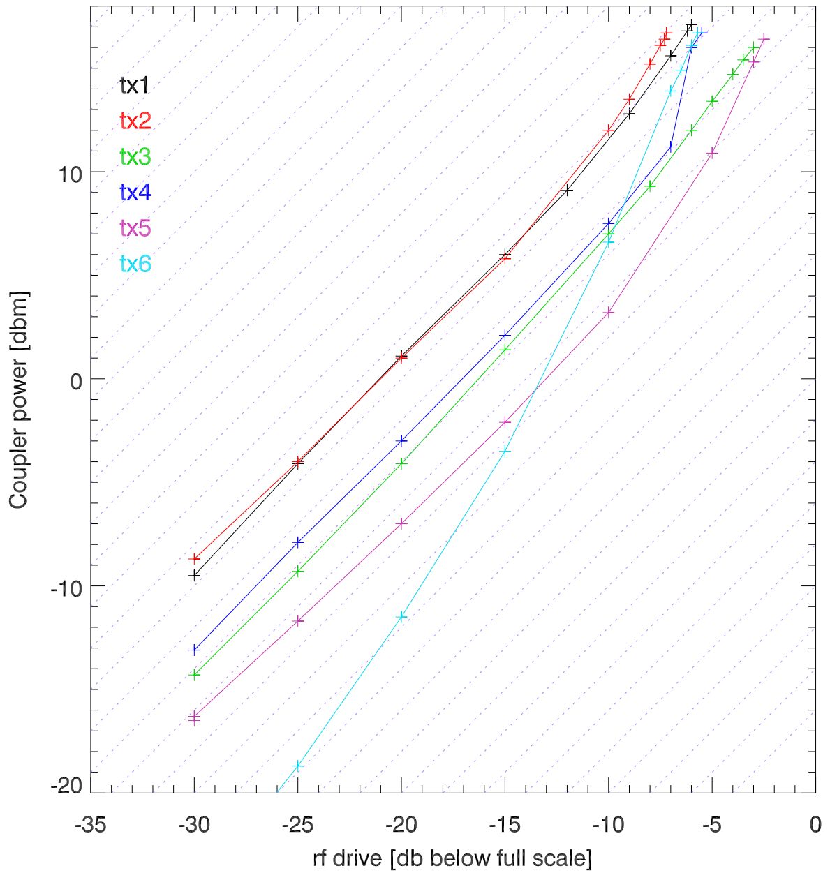
151102 on antenna. Output pwr vs rf drive (dbm vs dbf).
