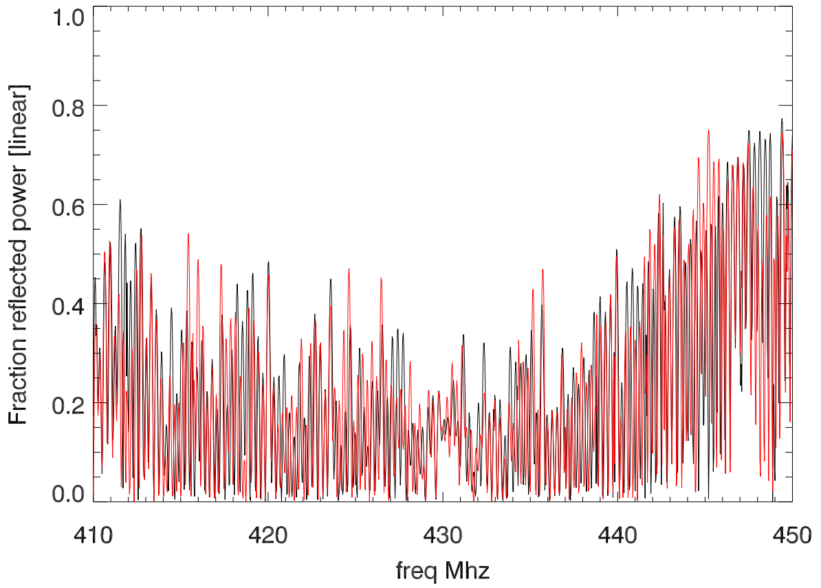
16jan12: Reflected power vs freq. ch in Tx mode
