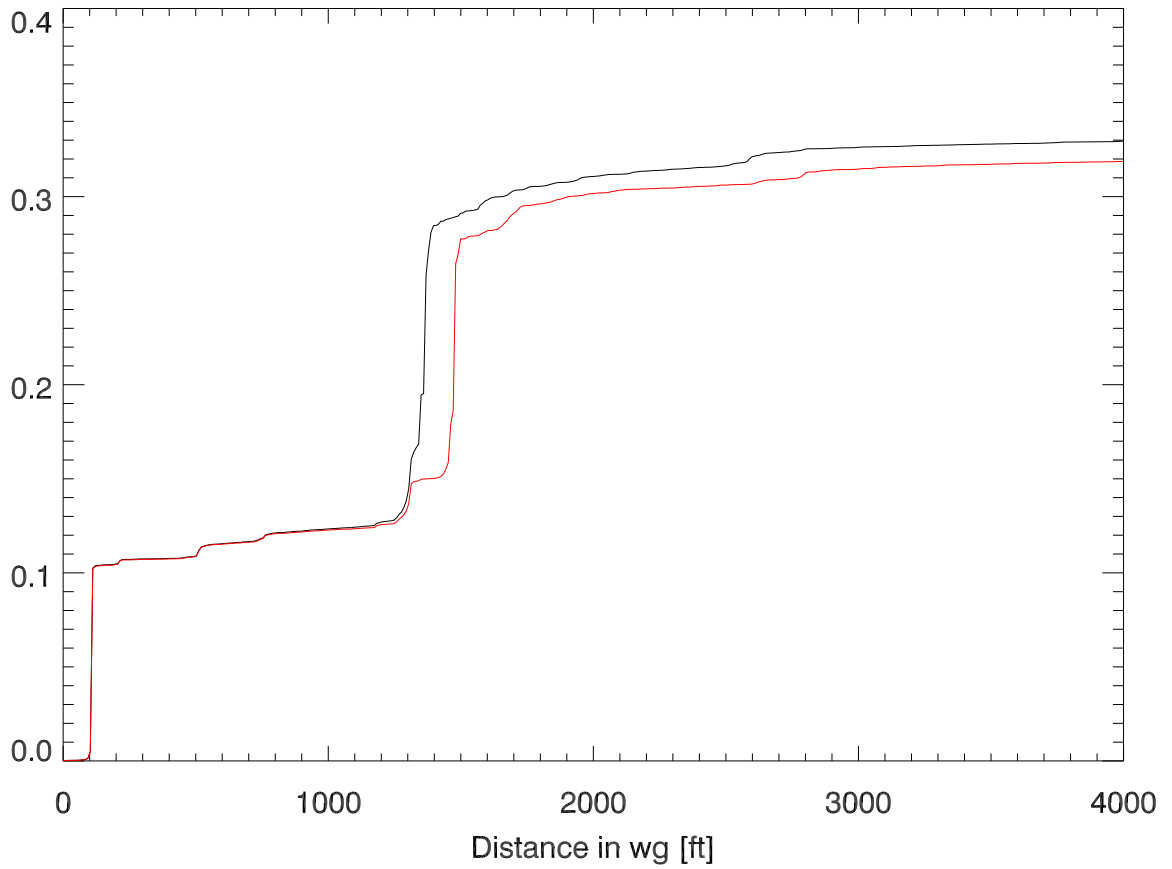
Cumulative reflected power vs distance
