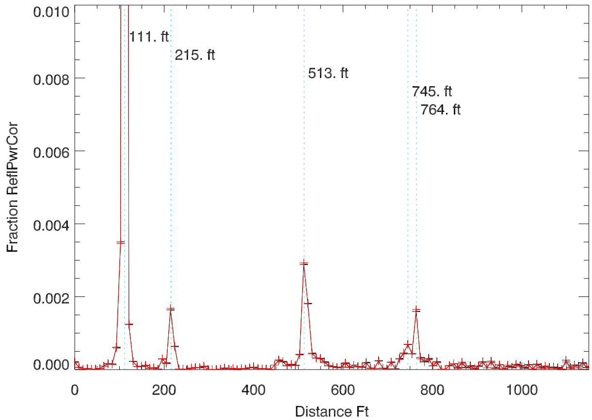
reflected power vs Distance. Blowup 0-1250 ft
