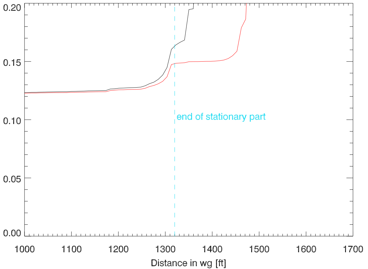
Cumulative reflected power vs distance
