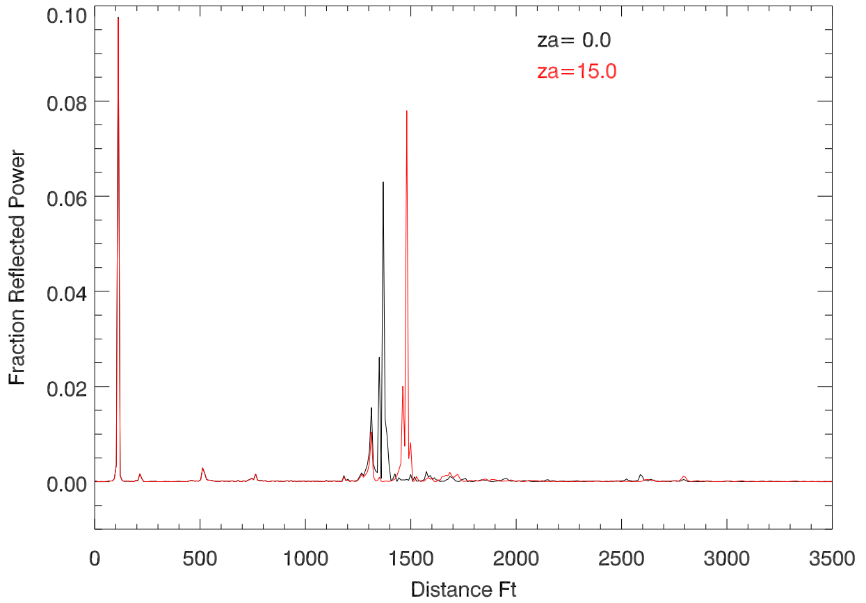
16jan12 reflected power vs Distance. CH Tx mode. Corrected
