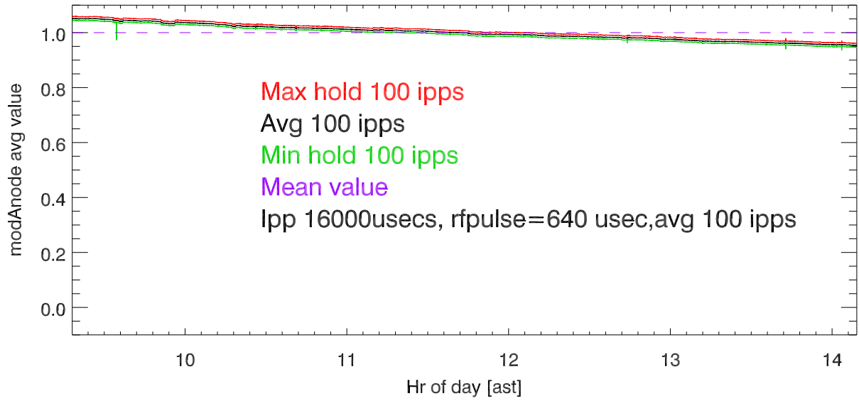
17dec19 430 Tx test. Avg Value ModeAnode vs time
