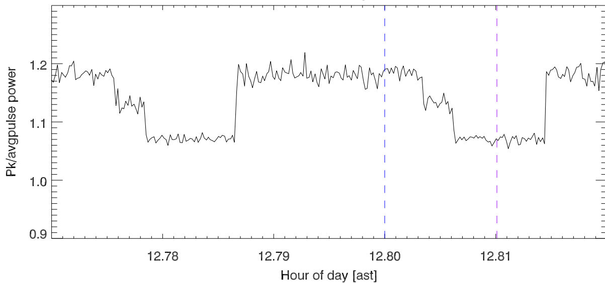
Ratio of PeakPulse/AvgPulse power
