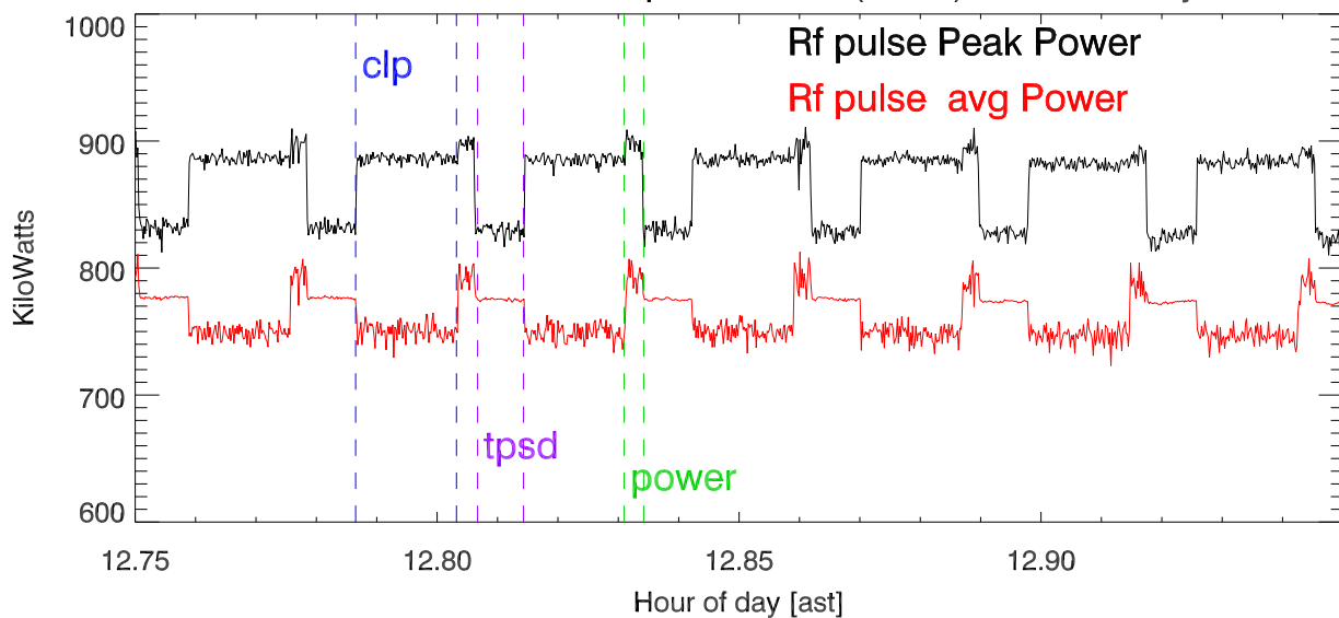
20191002 T3365 430tx power meter (dome) vs hour of day
