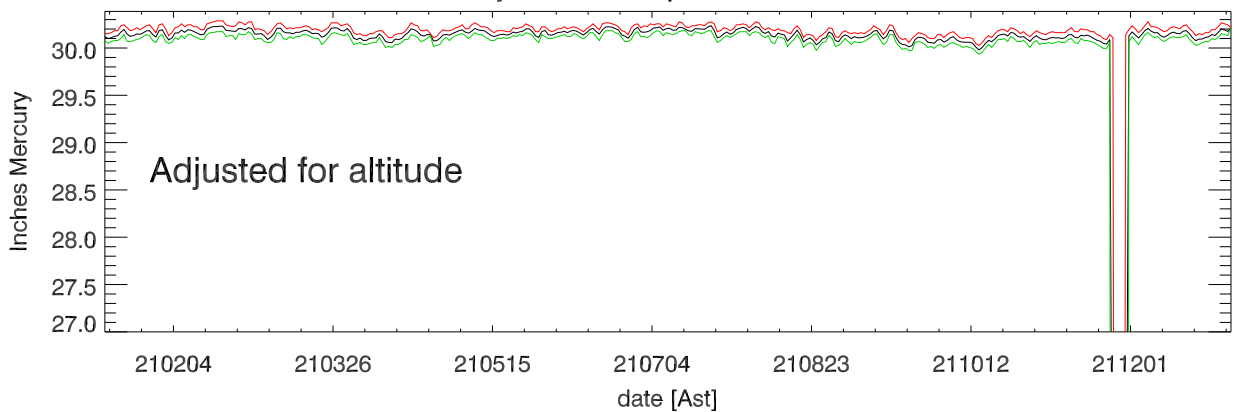
Daily barometric pressure vs date.
