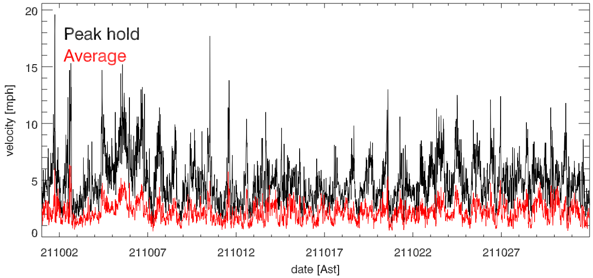
oct21 Avg & Peak velocities vs date (over 15.0 minutes)
