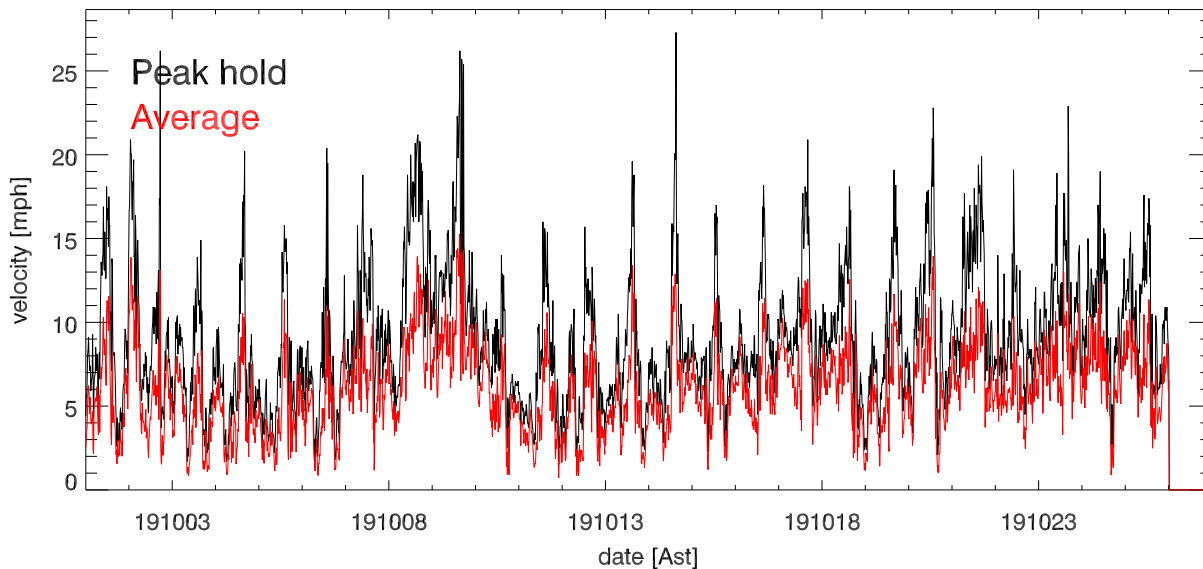
oct19 Avg & Peak velocities vs date (over 15.0 minutes)
