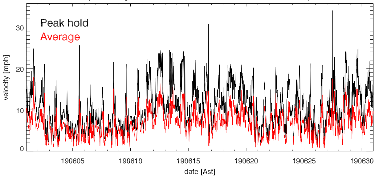
jun19 Avg & Peak velocities vs date (over 15.0 minutes)
