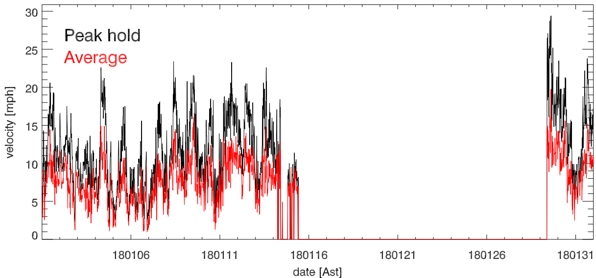
jan18 Avg & Peak velocities vs date (over 15.0 minutes)
