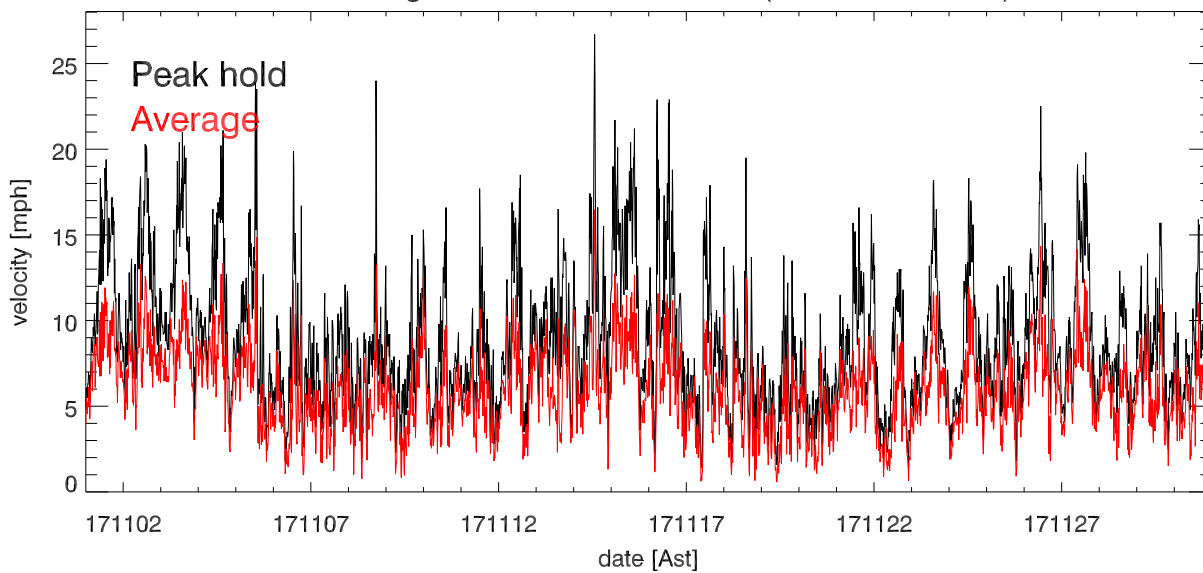
nov17 Avg & Peak velocities vs date (over 15.0 minutes)
