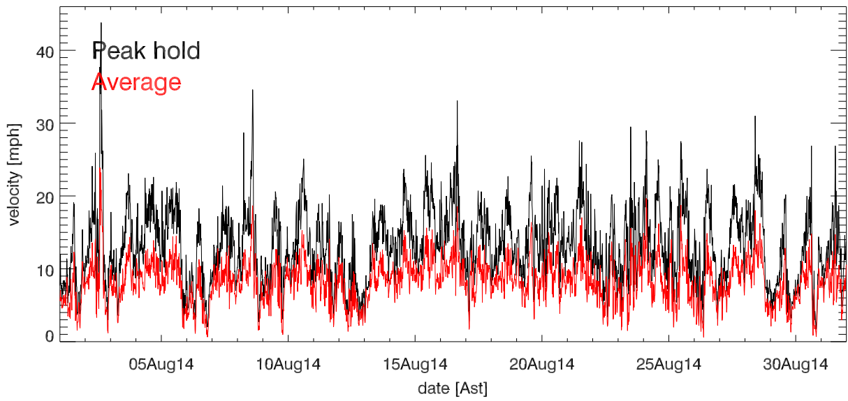
aug14 Avg & Peak velocities vs date (over 15.0 minutes)
