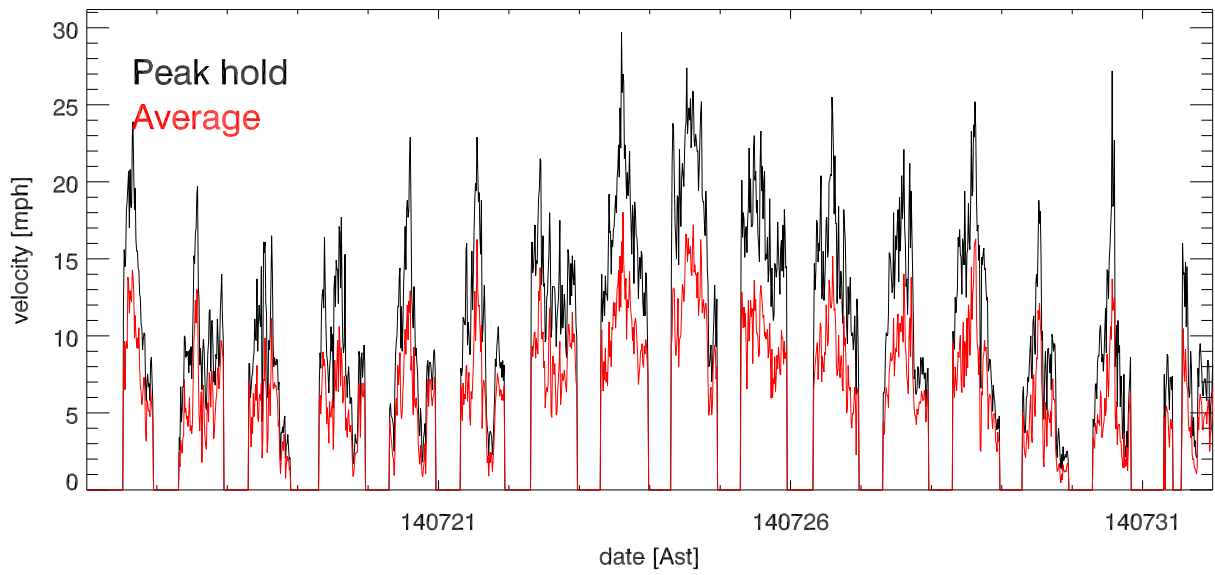
Jul14 Avg & Peak velocities vs date (over 15.0 minutes)
