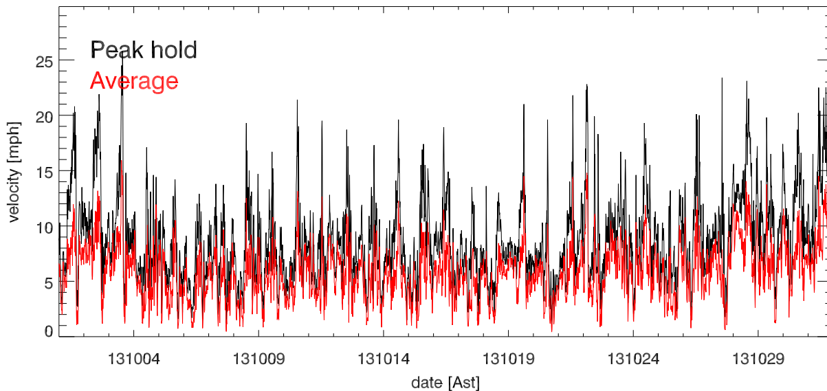
oct13 Avg & Peak velocities vs date (over 15.0 minutes)
