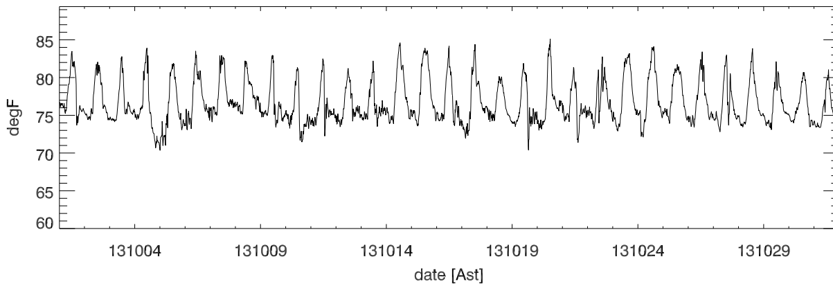
oct13 Temp vs date (averaged over 15.0 minutes)
