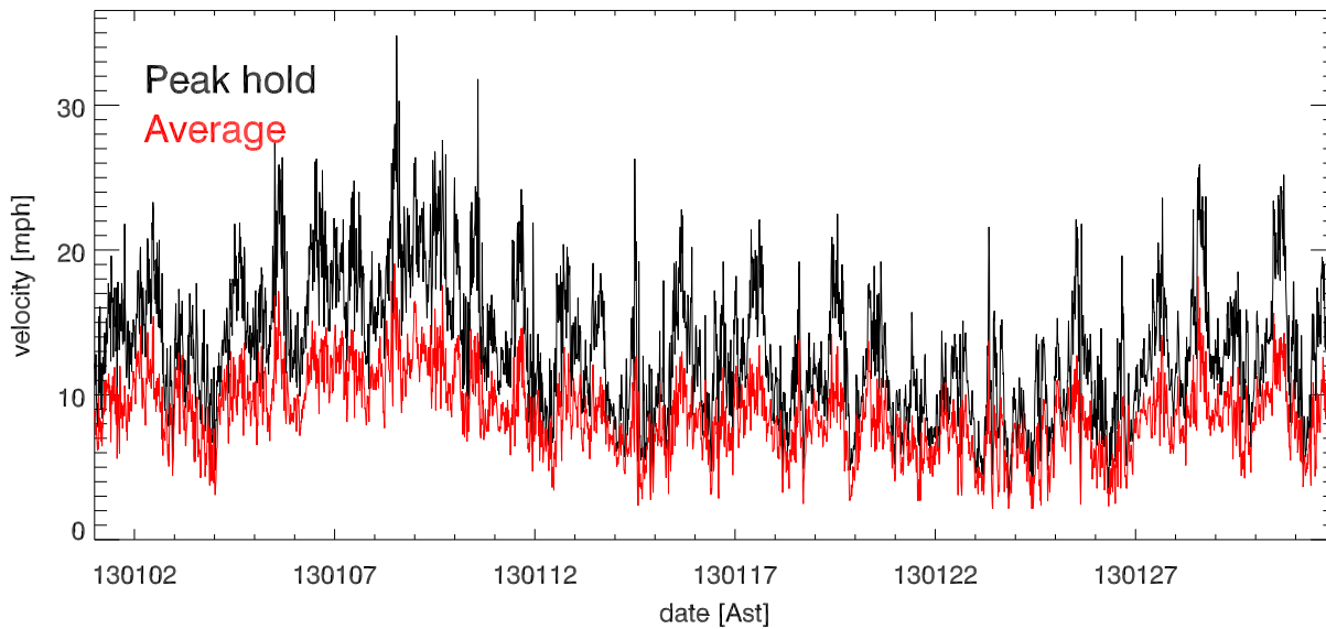
jan13 Avg & Peak velocities vs date (over 15.0 minutes)
