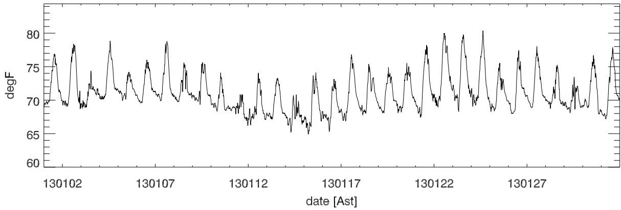
jan13 Temp vs date (averaged over 15.0 minutes)
