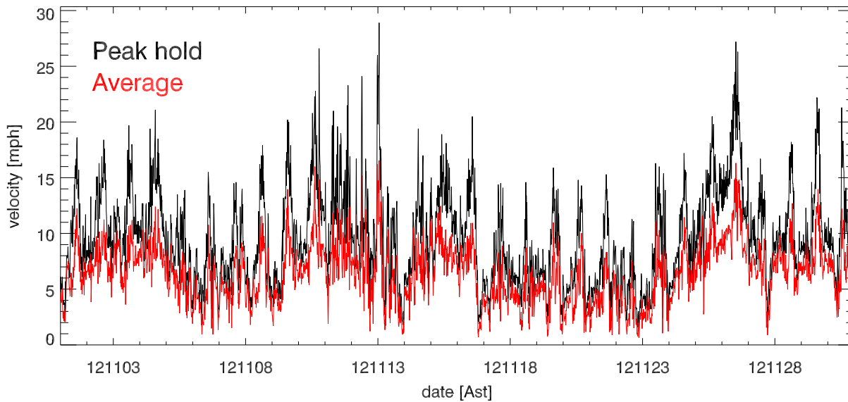
nov12 Avg & Peak velocities vs date (over 15.0 minutes)
