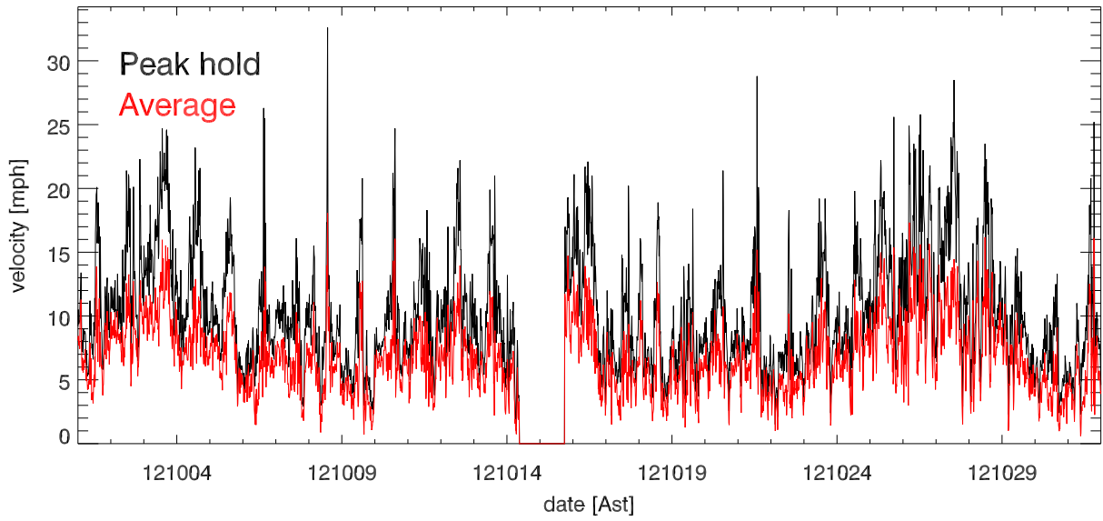
oct12 Avg & Peak velocities vs date (over 15.0 minutes)
