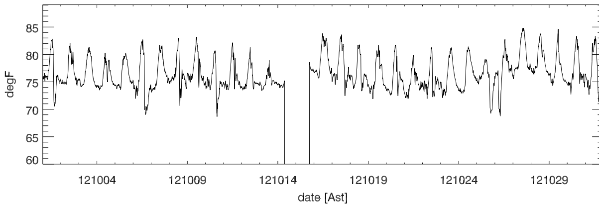
oct12 Temp vs date (averaged over 15.0 minutes)
