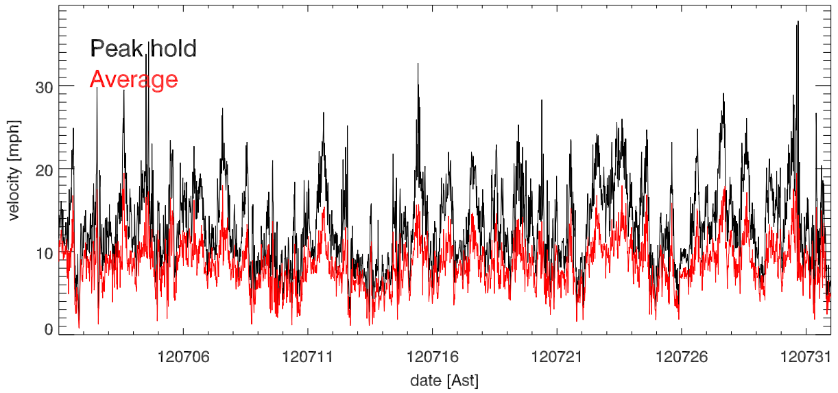
Jul12 Avg & Peak velocities vs date (over 15.0 minutes)
