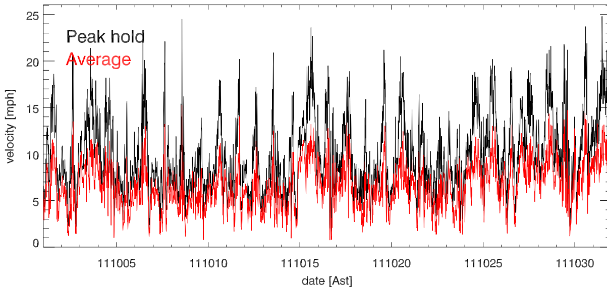
oct11 Avg & Peak velocities vs date (over 15.0 minutes)
