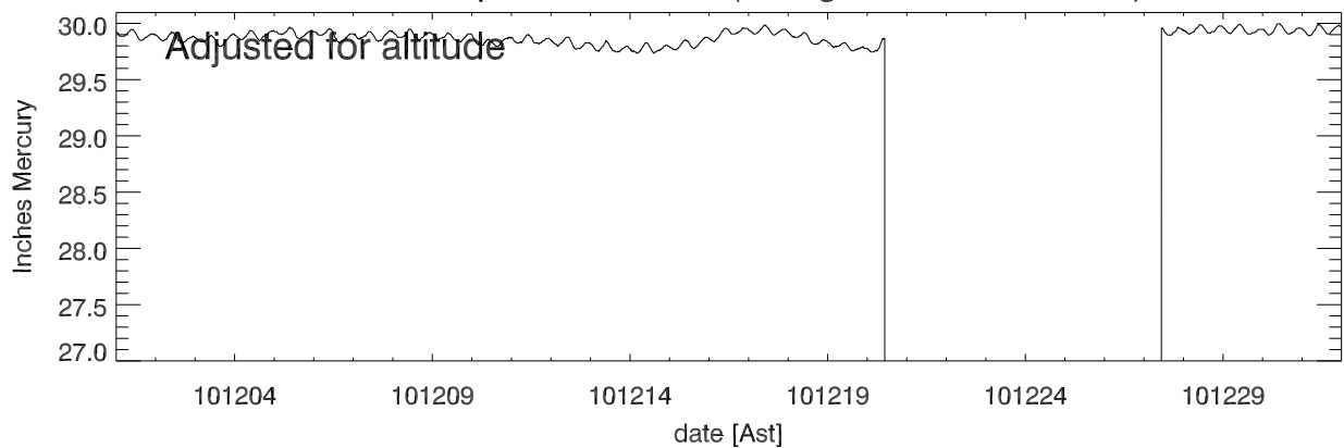
Barometric pressure vs date. (averaged over 15.0 minutes)
