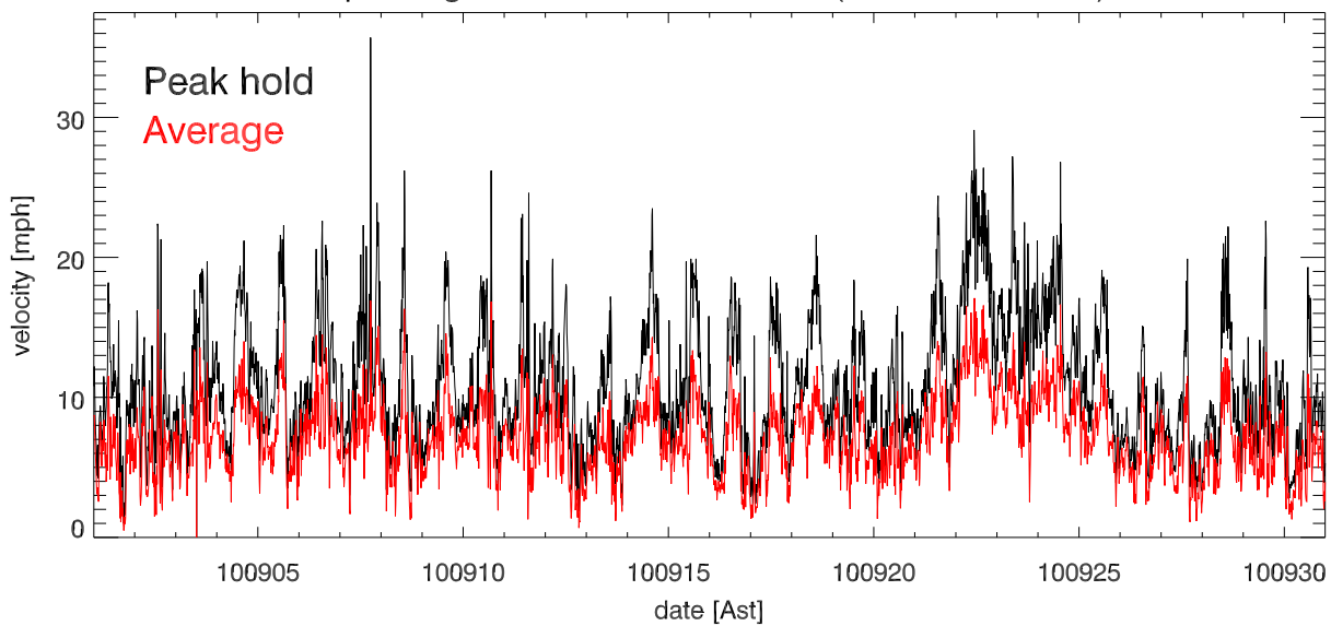
sep10 Avg & Peak velocities vs date (over 15.0 minutes)
