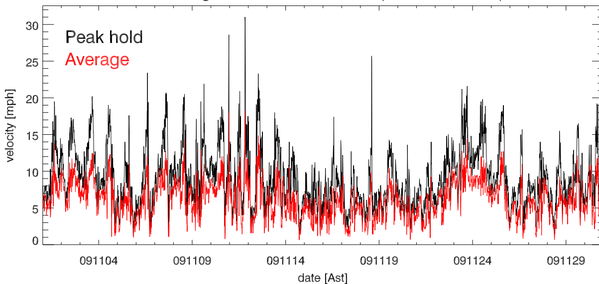
nov09 Avg & Peak velocities vs date (over 15.0 minutes)
