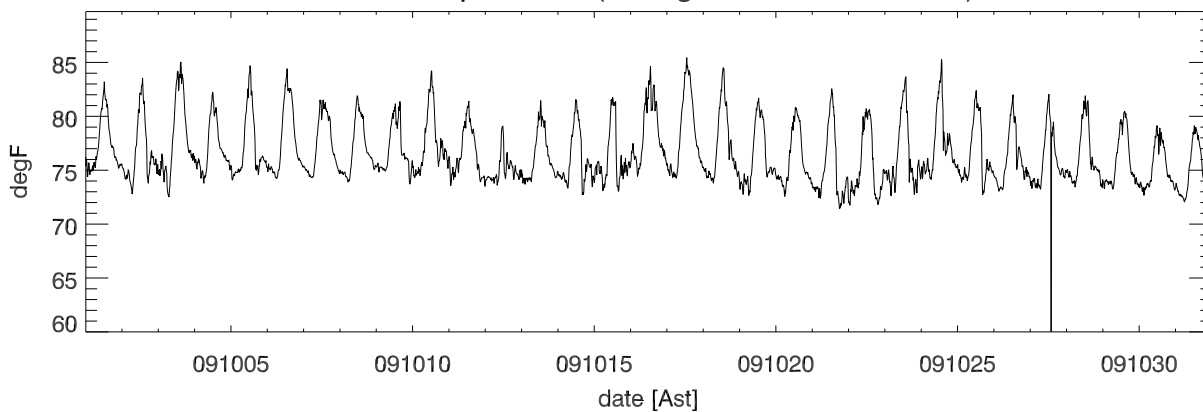
oct09 Temp vs date (averaged over 15.0 minutes)
