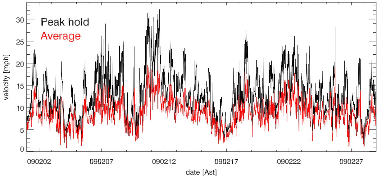
feb09 Avg & Peak velocities vs date (over 15.0 minutes)
