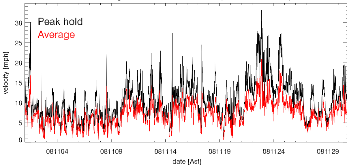
nov08 Avg & Peak velocities vs date (over 15.0 minutes)
