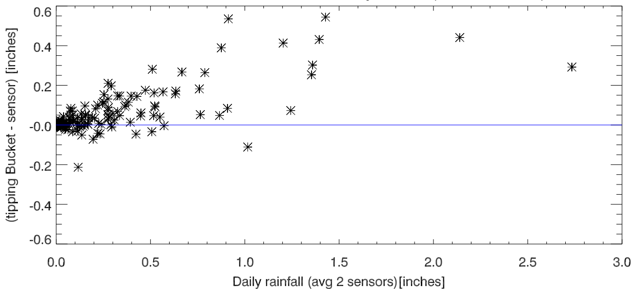
measurement difference vs daily rainfall (bucket-sensor)
