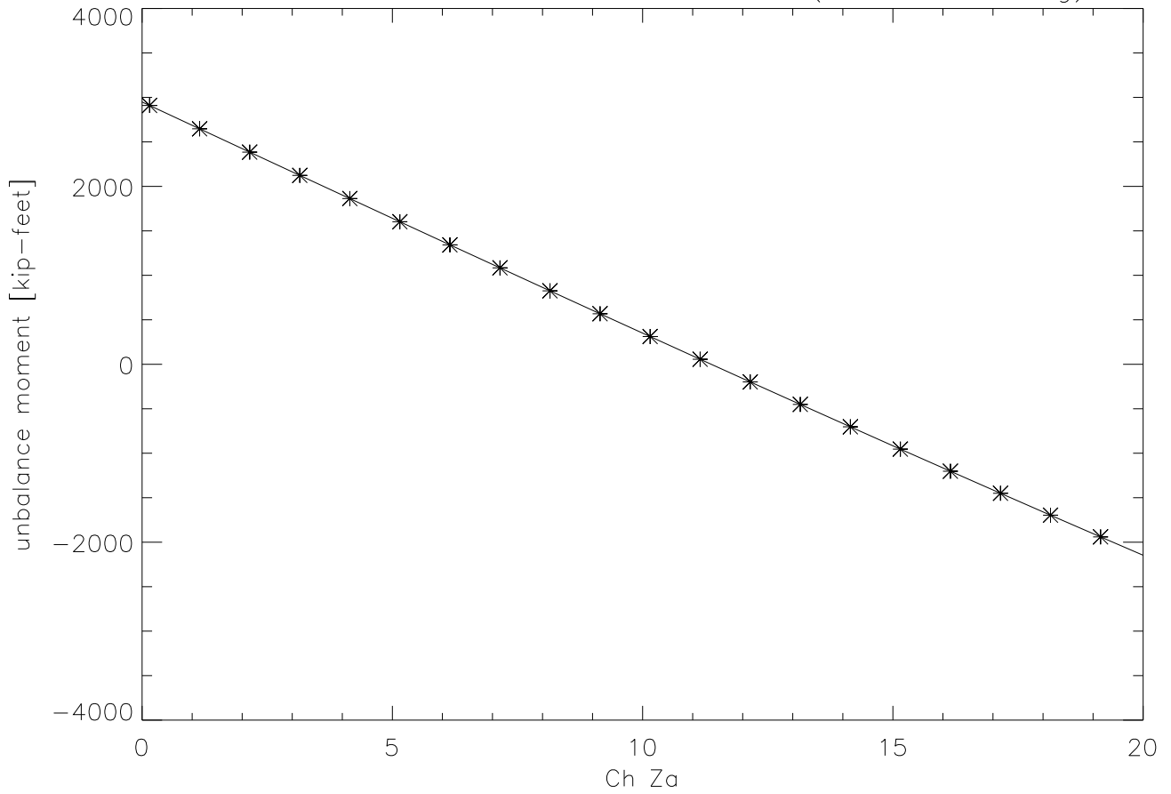
az arm unbalanced moment vs Ch za (dome at 8.4deg)
