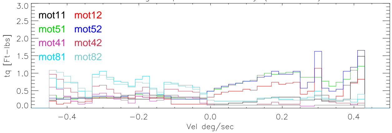
avg torques vs velocity (group 1)
