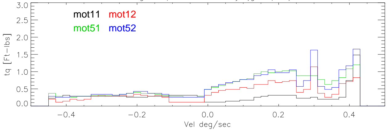
avg torques vs velocity (group 2)
