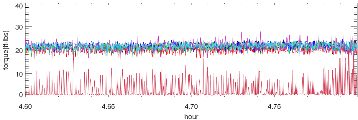
Dome torques vs hour of day
