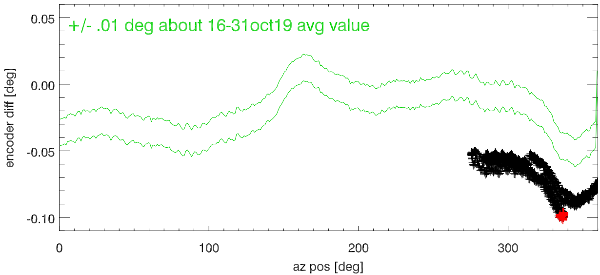
Az encoder difference vs azimuth position 0-8.9am 191016
