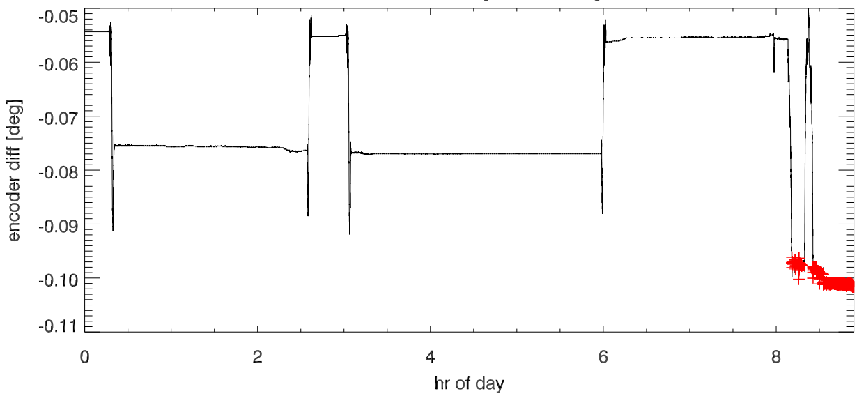
Az encoder difference [enc1-enc2] vs hour
