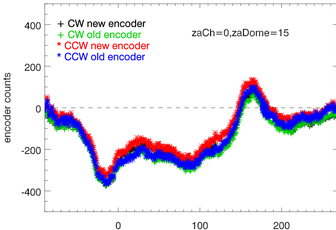
17jan13 az encoder difference before/after encoder 2 replaced
