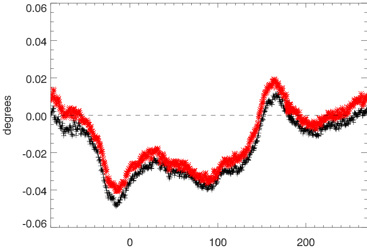
22jan13 az encoder difference after encoder 2 replaced
