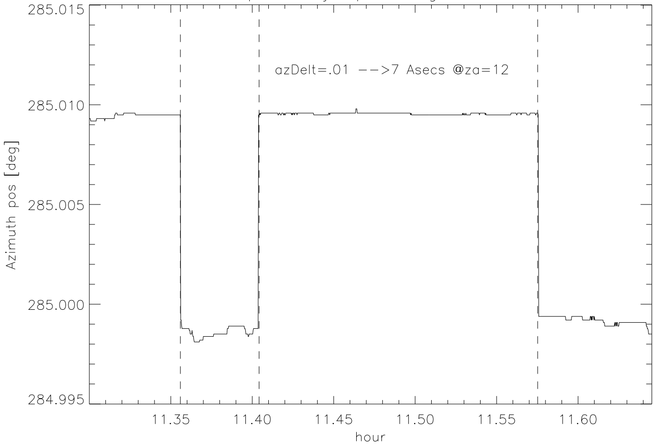
Azimuth position jumps during encoder 1 fail
