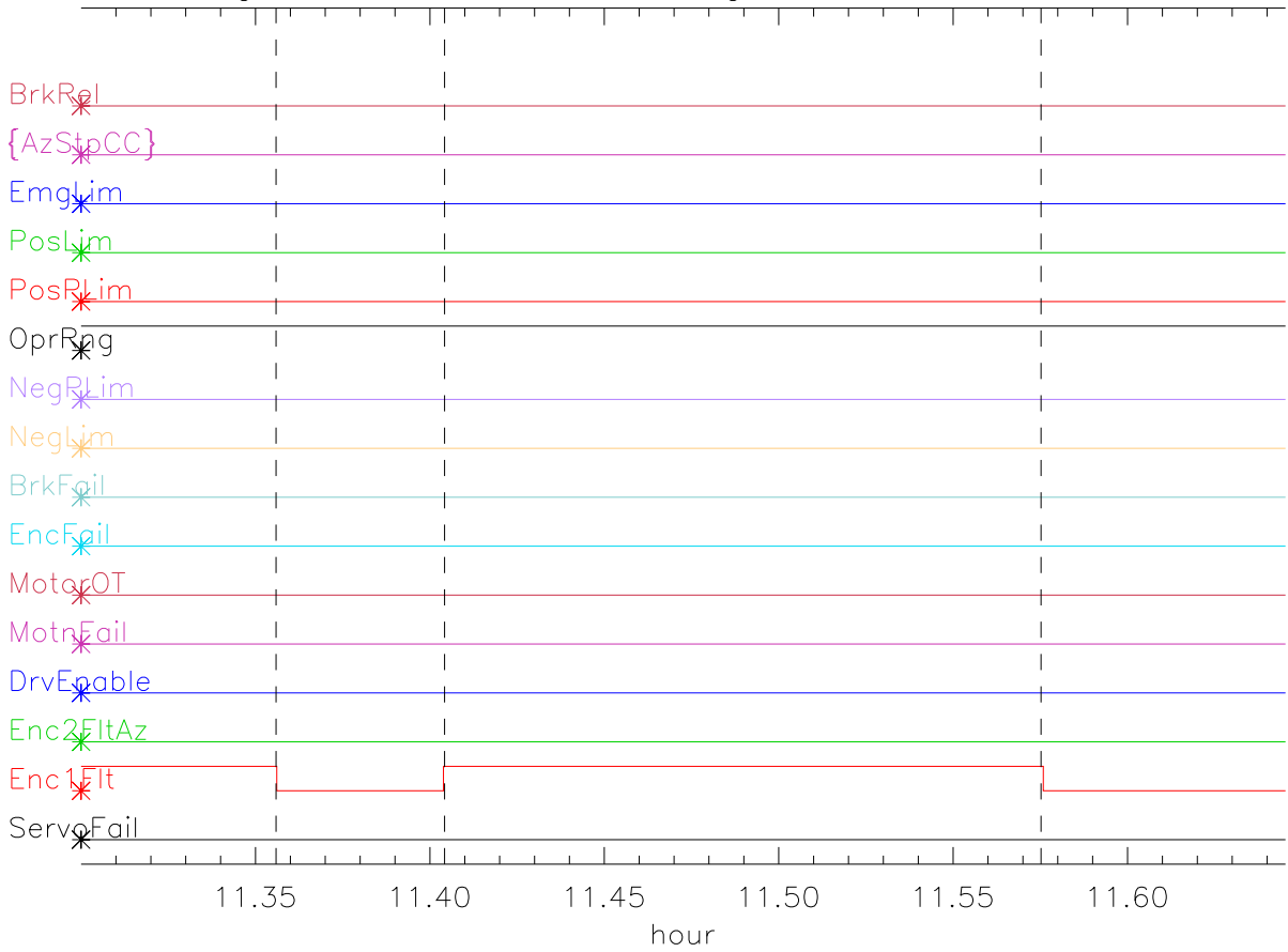
Azimuth position jumps during encoder 1 fail
