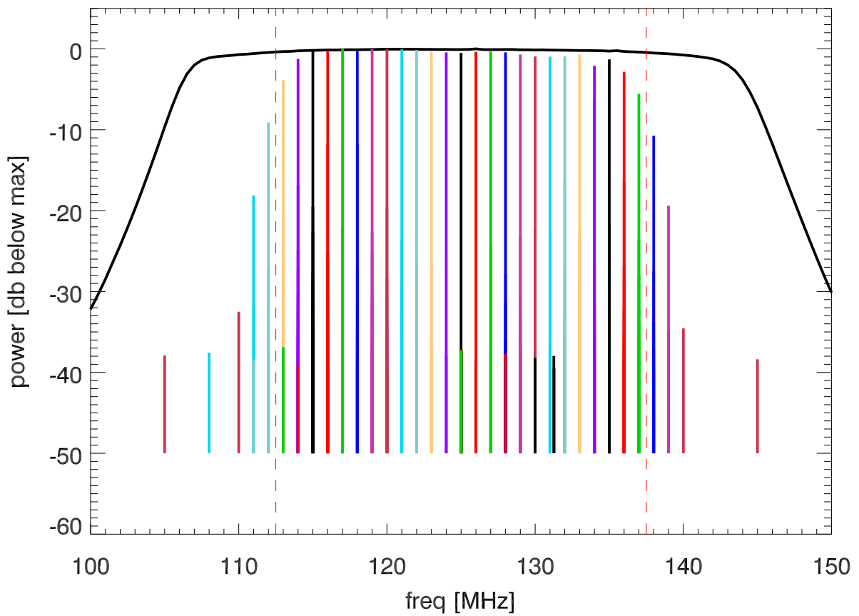
sweep 105->145, no filter
