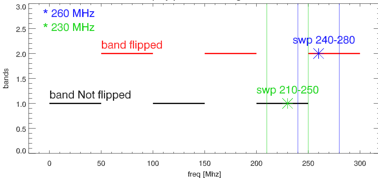
50 Mhz usrp nyquist zones using basic rx board
