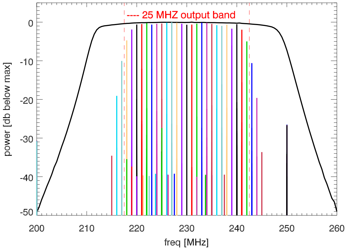
230 MHz filter used and measured values
