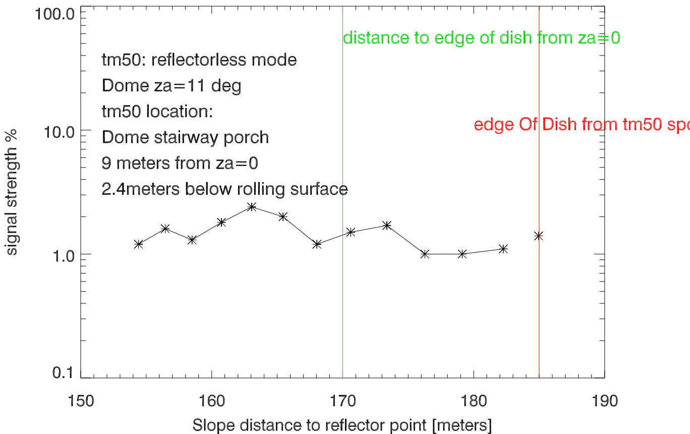
06feb20 tm50 signal strength from platform vs slope distance
