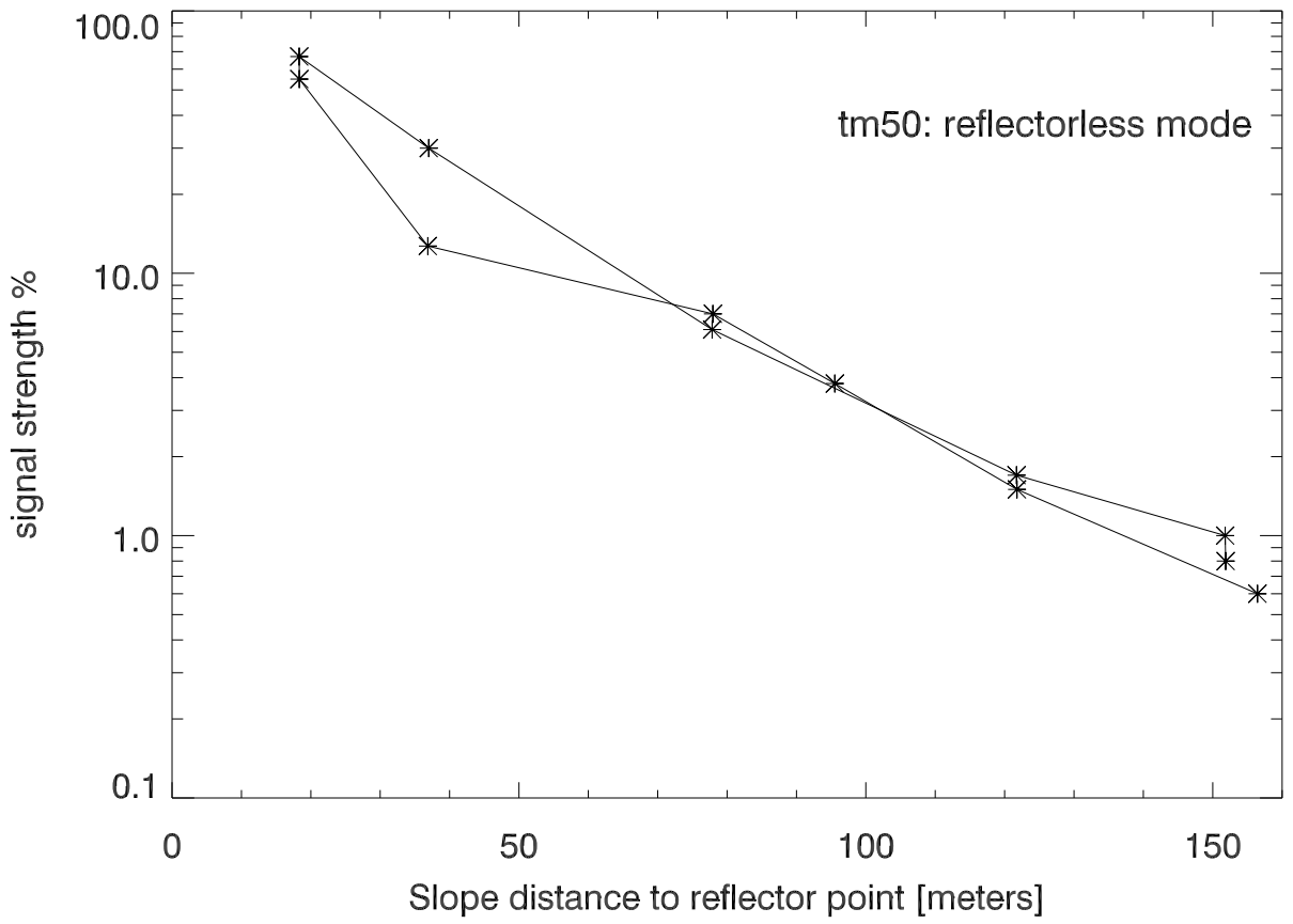
29jan20 tm50 signal strength from ao9 to reflector. slope distance
