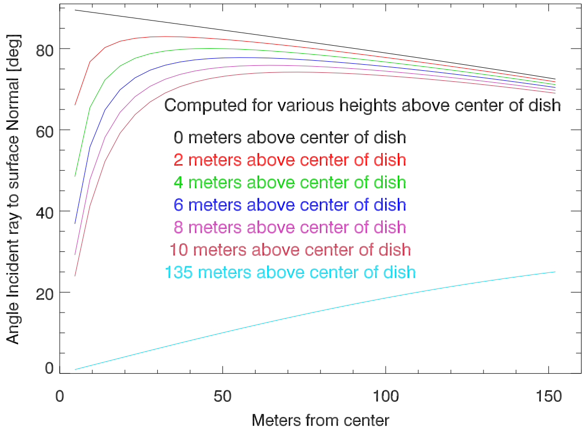
Angle to surface Normal vs distance from center
