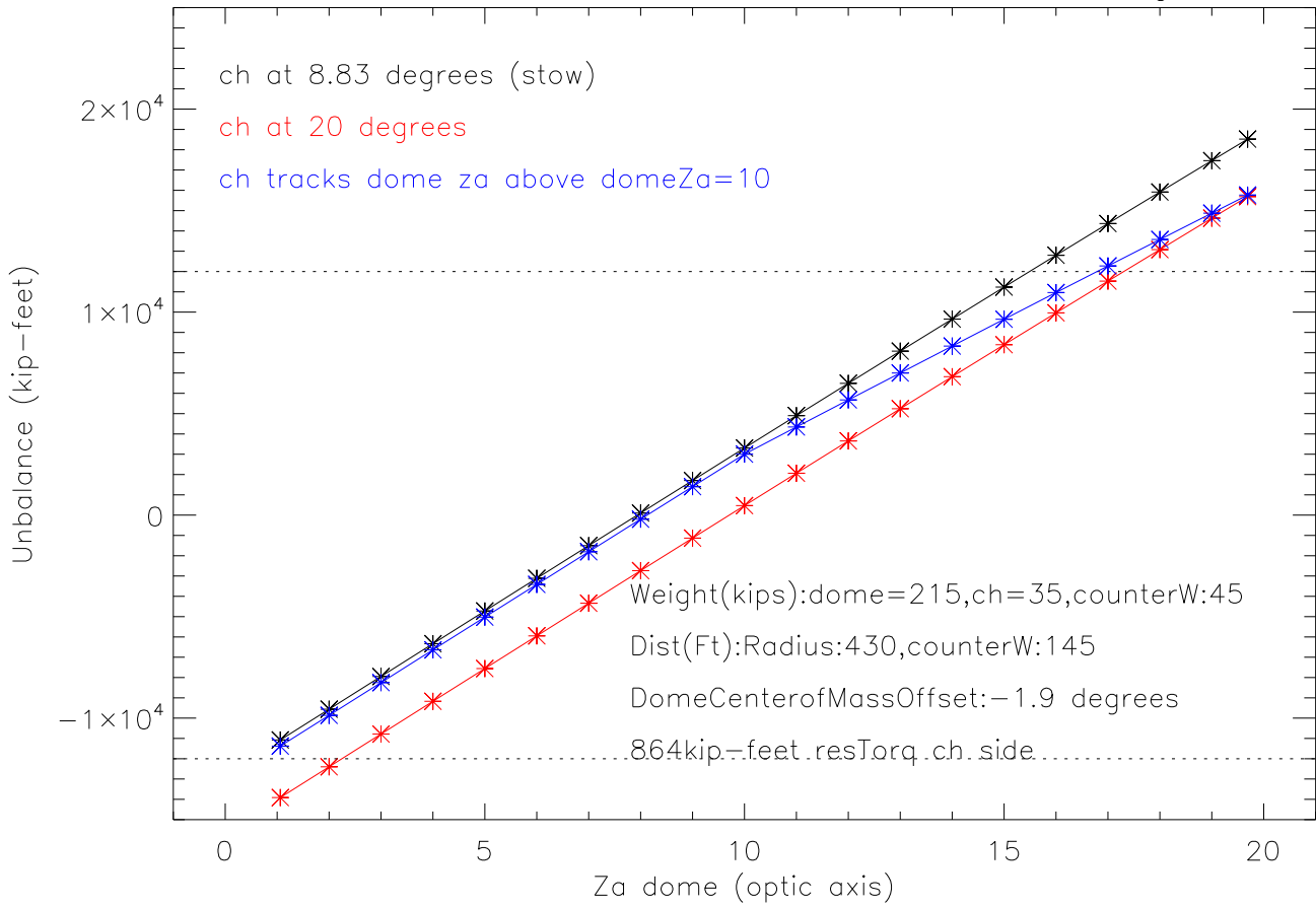
Unbalanced moment: dome fixed, ch moves
