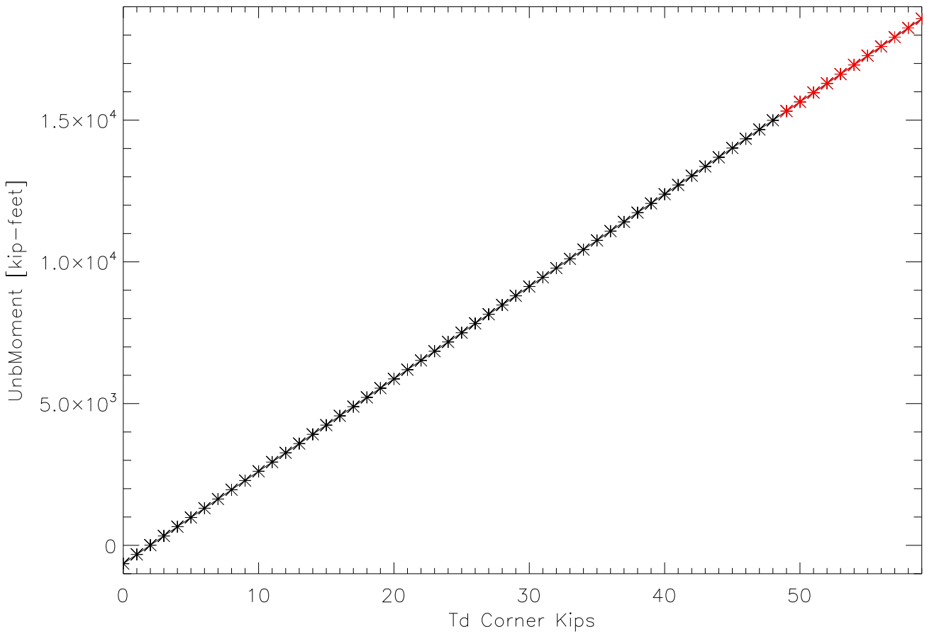
Max unbalanced moment vs td corner tension
