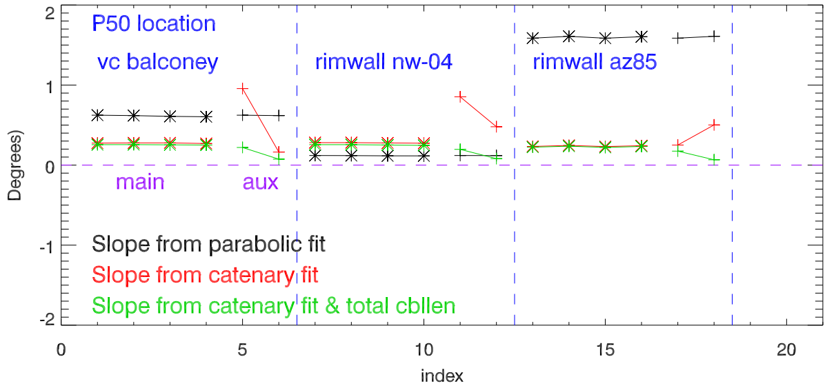
Platform cable slope dif (measured - drawings). Tower 12
