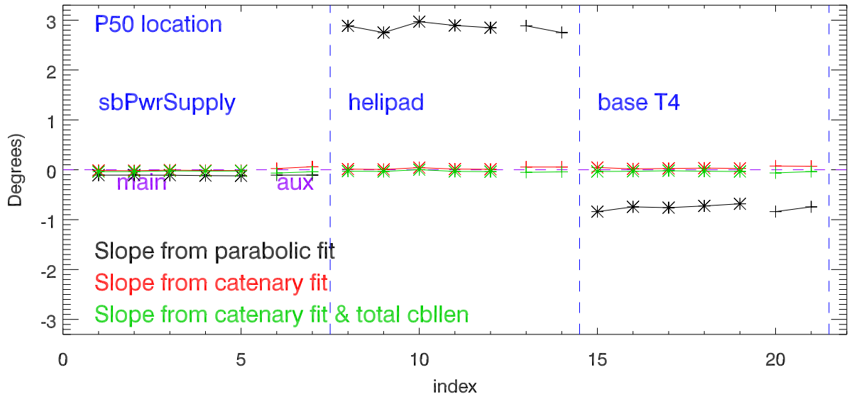
Backstay cable slope dif (measured - drawings). Tower 12
