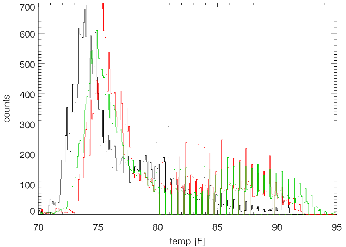
Histogram of Backstay cable temperatures
