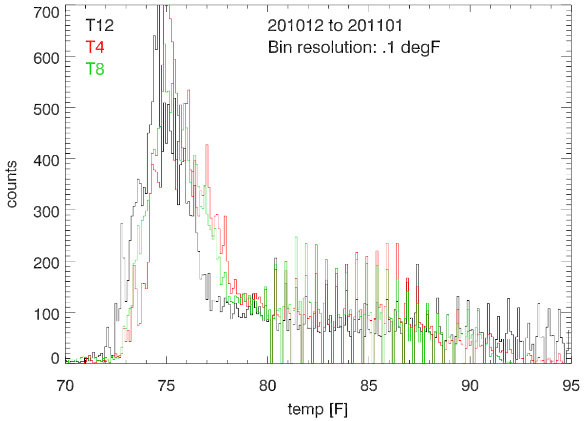
Histogram of Platform cable temperatures
