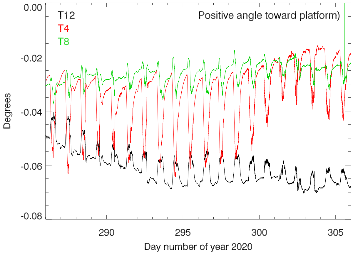
Tower tilt sensor Radial angle vs date (201012 to 201101)
