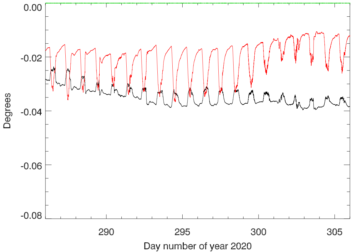
Tower tilt sensors tangential angle vs date
