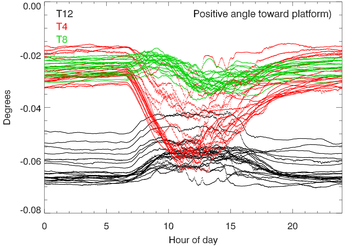
Tower tilt sensor Radial angle vs Hr of day (201012 to 201101)
