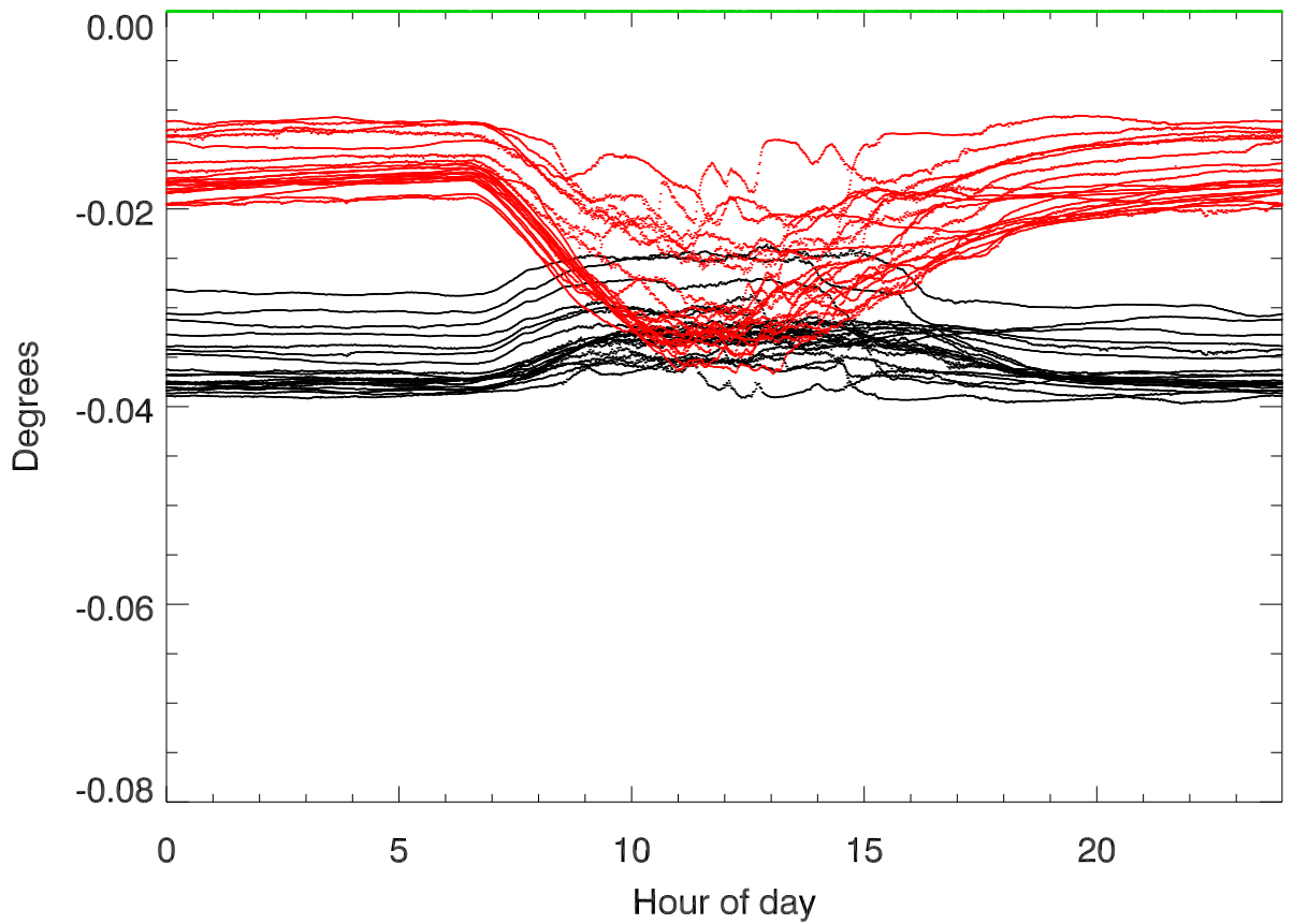
Tower tilt sensors tangential angle vs Hr of day
