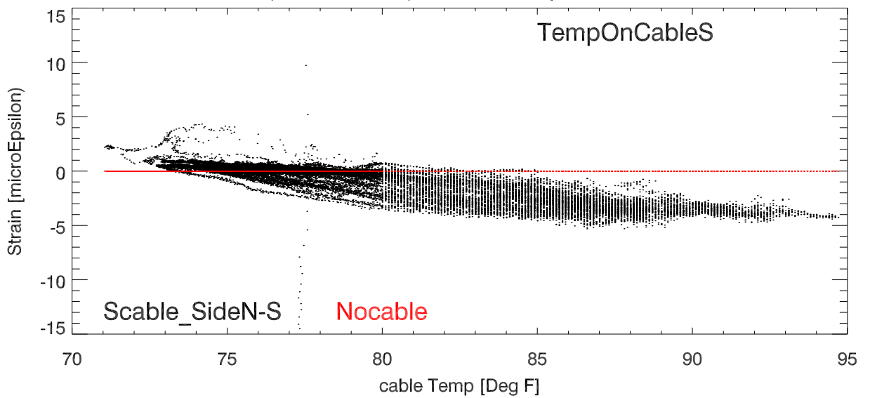
StrainDif (Side1 - Side2) vs cable temp. Platform Tower 4
