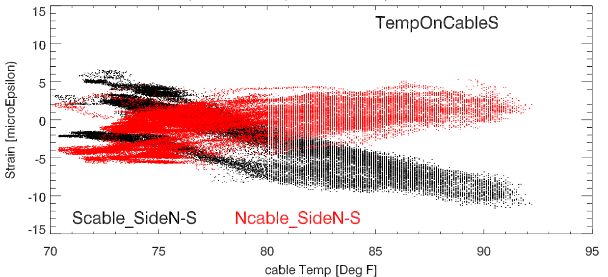
StrainDif (Side1 - Side2) vs cable temp. Platform Tower 8
