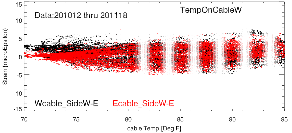
StrainDif (Side1 - Side2) vs cable temp. Platform Tower 12
